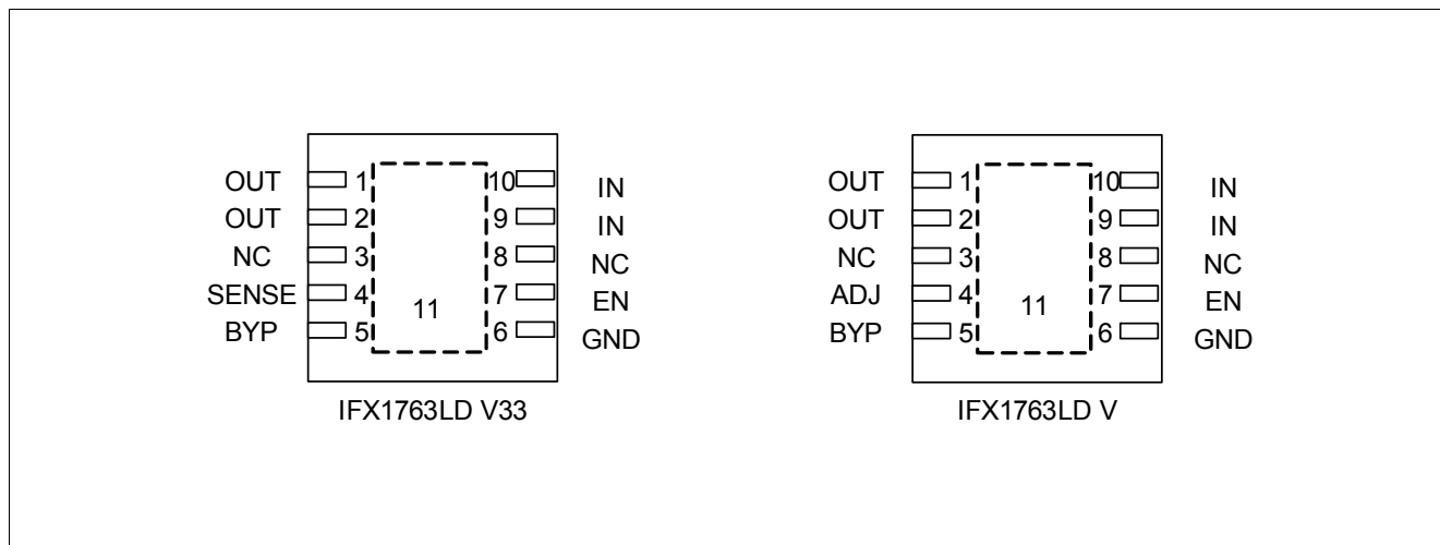
Figure 4 Pin Configuration of IFX1763 in PG-TSON-10 for fixed voltage and adjustable version
